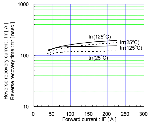
Reverse recovery characteristics (typ.) V_{cc}=600\text{V} , V_{GE}=\pm 15\text{V} , R_G=4.7\Omega
