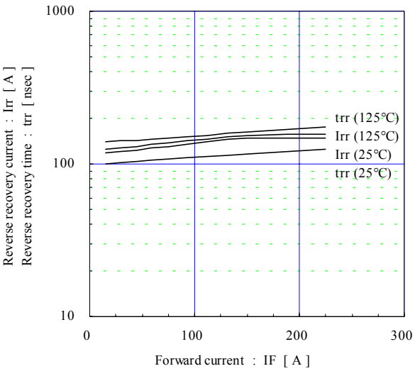
Reverse recovery characteristics (typ.) Vcc=600V, VGE=+15V, Rg=22 ohm
