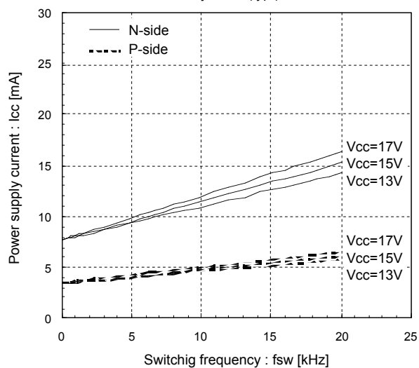
Power supply current vs. Switching frequency T J =25°C (typ.)
