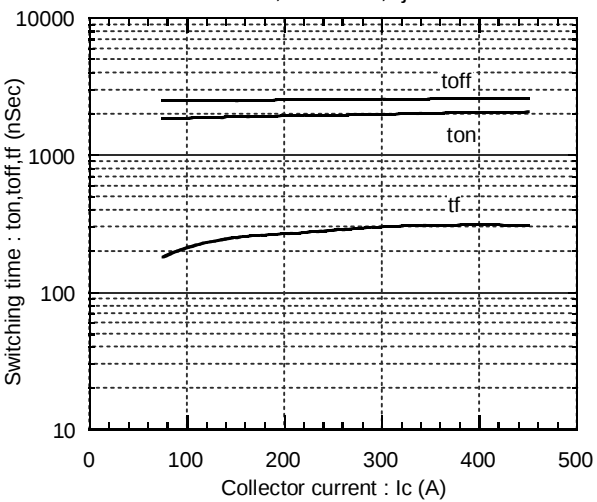
Switching time vs. Collector current Edc=300V,Vcc=15V,Tj=125°C
