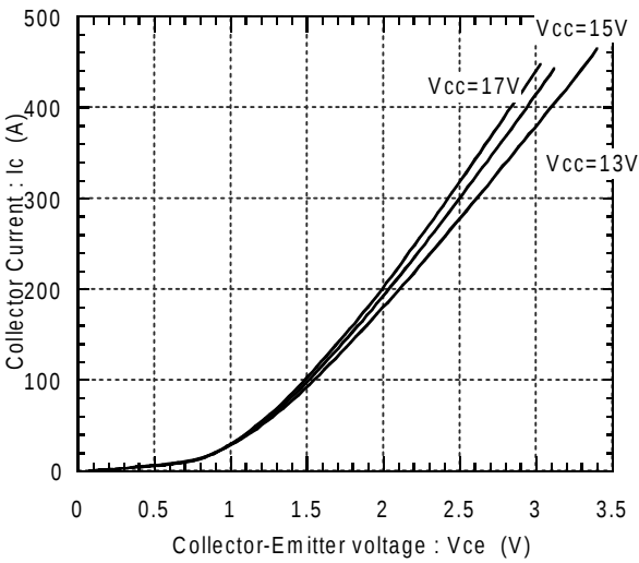
Collector current vs. Collector-Emittter voltage Tj=125°C
