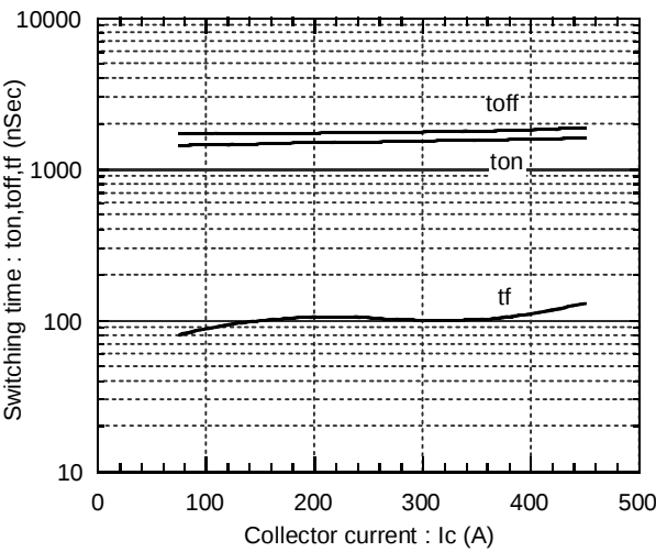
Switching time vs. Collector current Edc=300V,Vcc=15V,Tj=25°C
