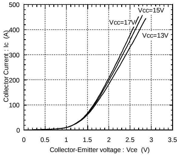
Collector current vs. Collector-Emittter voltage Tj=25°C
